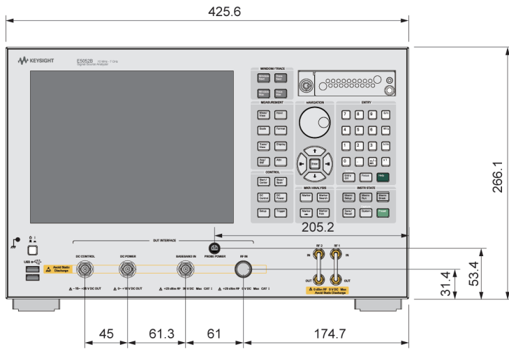
Figure 8-1. Front view
