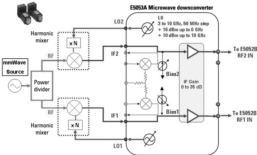
Figure 10-4. System set-up for harmonic mixers (E5053A + E5052B)
