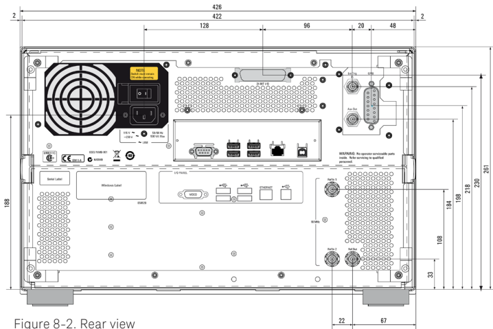
Figure 8-2. Rear view
