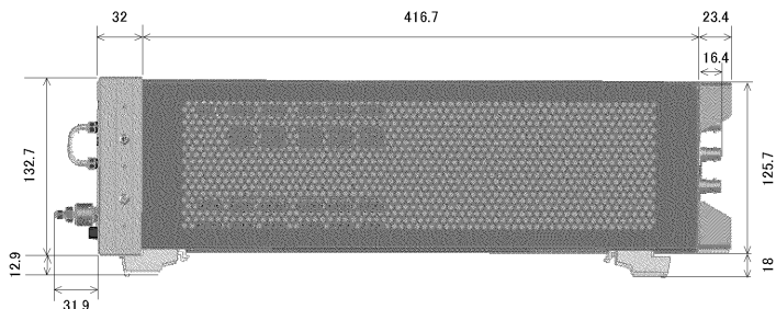
Figure 10-8. Side view
