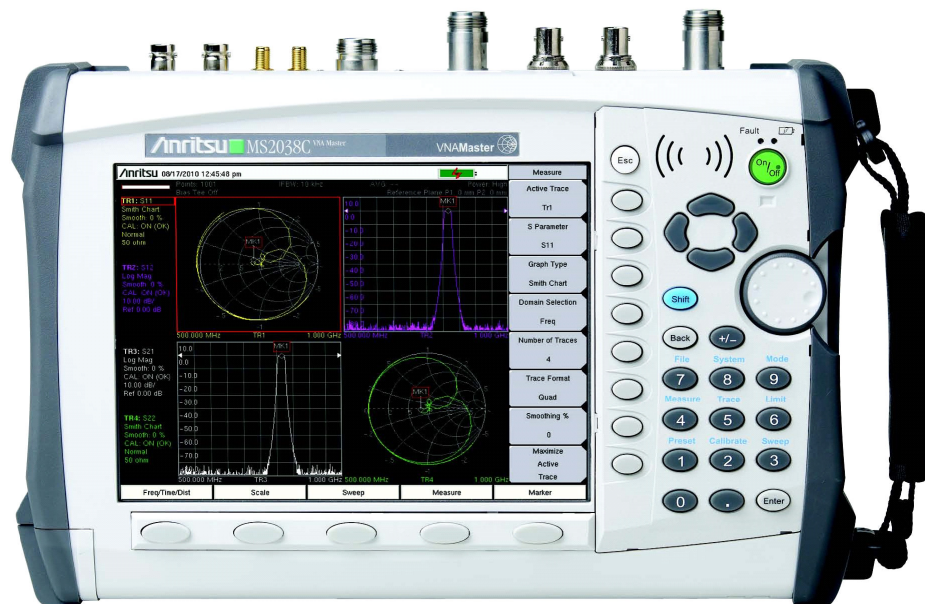
VNA Master™ MS202xC/MS203xC Vector Network Analyzer + Spectrum Analyzer Size: 315 mm x 211 mm x 78/97mm (12.4 in x 8.3 in x 3.1/3.8 in), Lightweight: 4.5 kg to 4.8 kg (9.9 lb to 10.5 lb)
