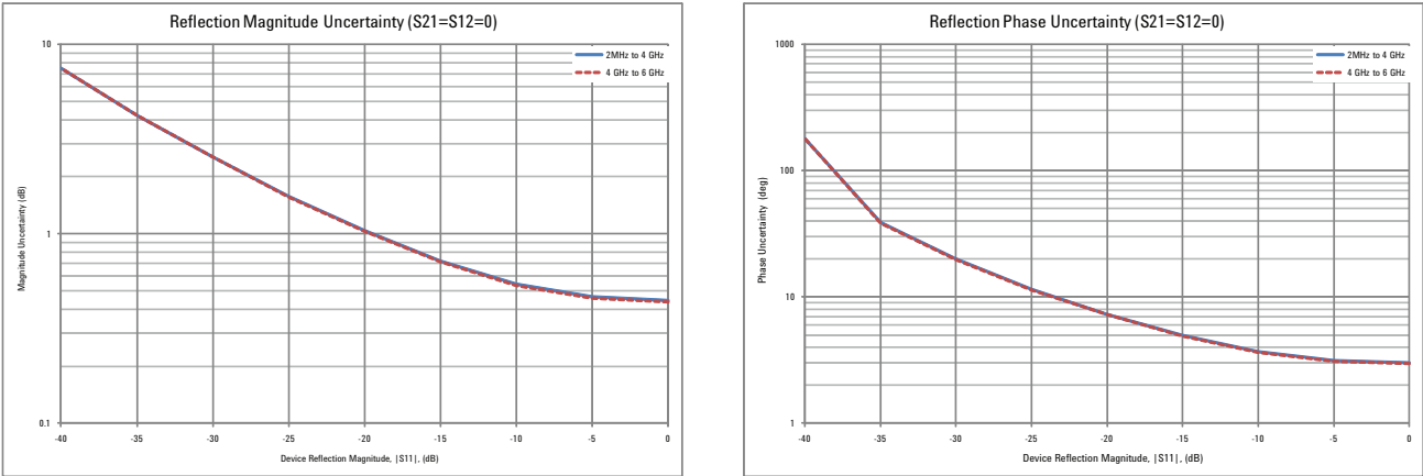
Figure 4: Reflection uncertainty (specification)
