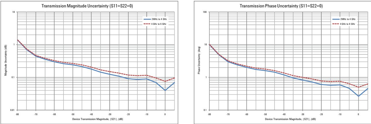
Figure 1: Transmission uncertainty (specification)
