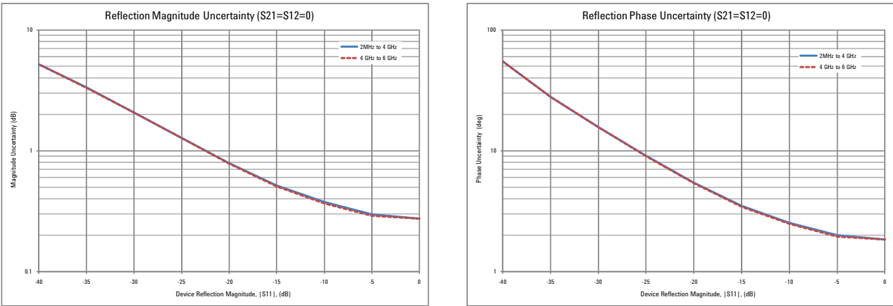
Figure 2: Reflection uncertainty (specification)
