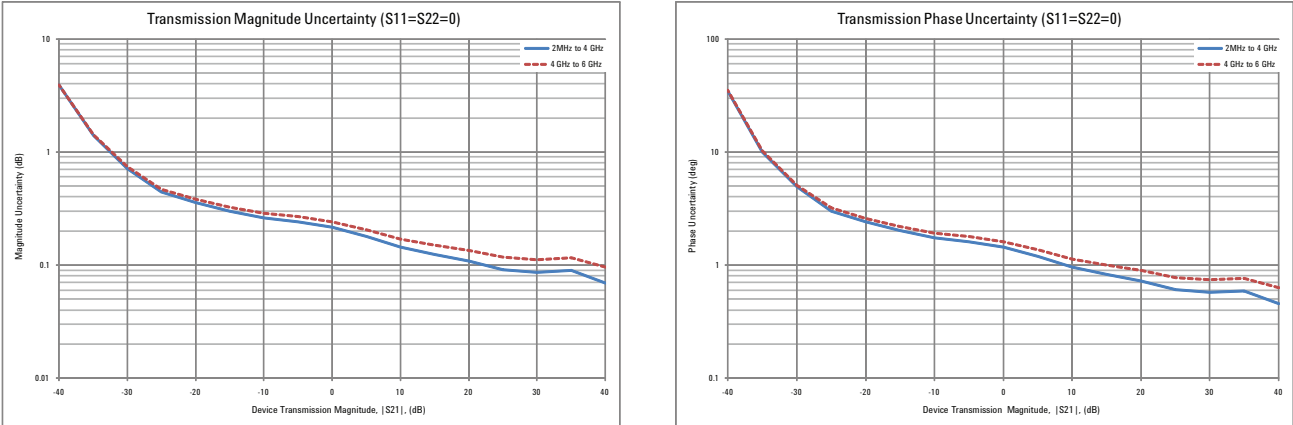
Figure 3: Transmission uncertainty (specification)
