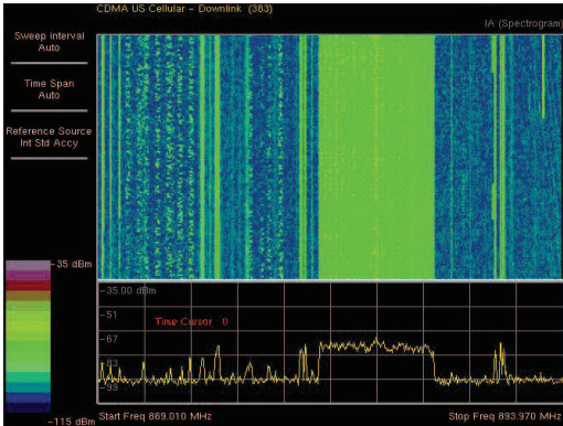
With Option 25, spectrogram measurements identifies intermittent interference.
