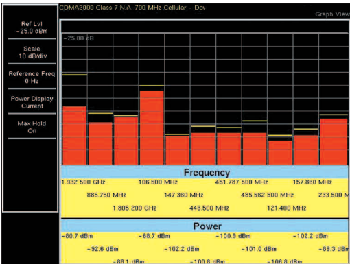
With Option 27, channel scanner measures power of multiple transmitters.
