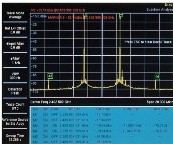
Signal Measurements
