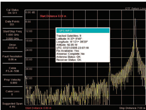
GPS Receiver
