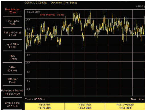
With Option 25, RSSI measurement analyzes signal strength of a signal over time.
